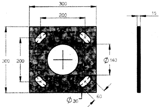
BASE PLATE DETAIL SCALE 1 : 8
